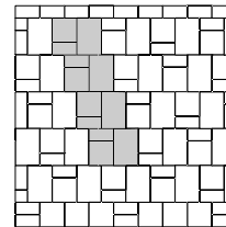
Pattern 5 Two full layers
