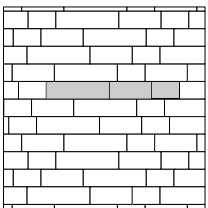
Pattern 1 Small = 21% Medium = 31.5% Large = 47.4%
