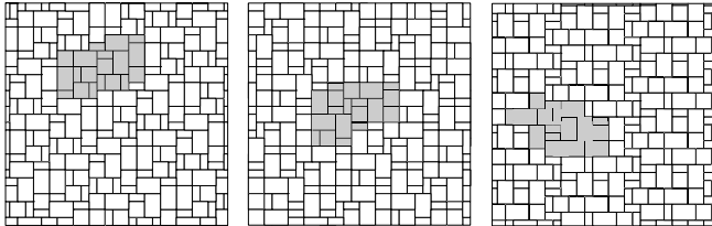
Patterns shown use one complete pallet layer.
