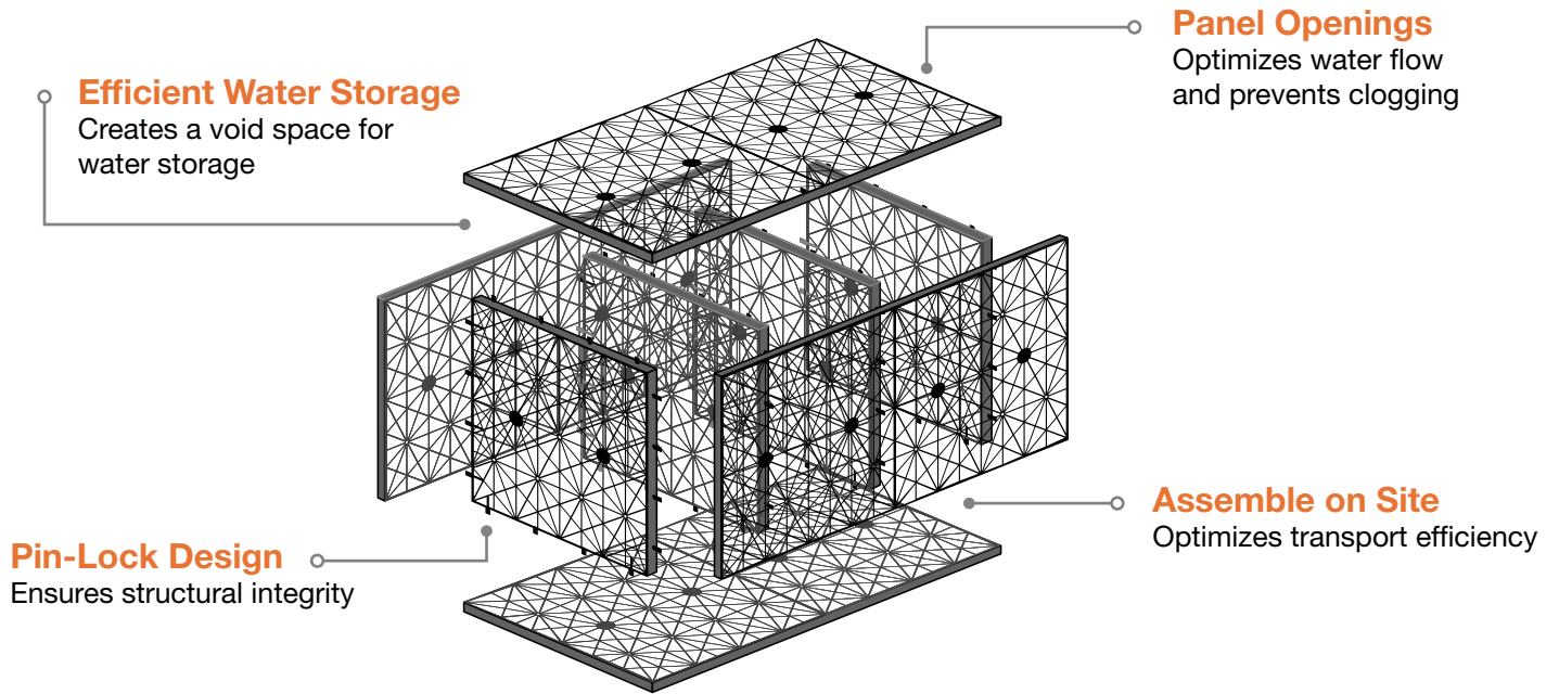
Compare AquaBlox® Water Storage Modules
