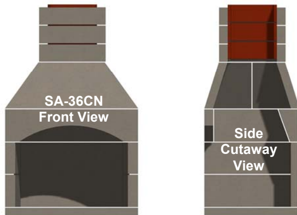
Figure 1. SA-36CN Fireplace Assembly & Cutaway View
