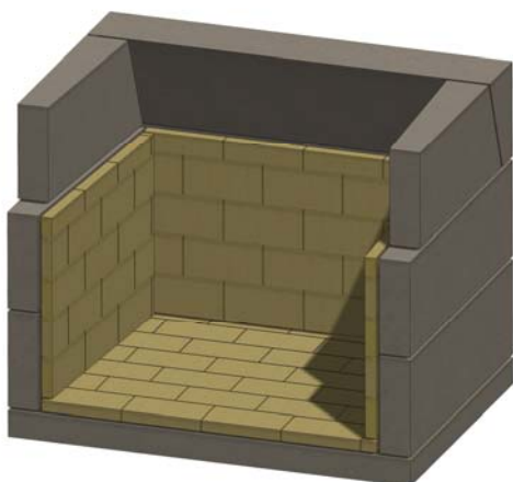
Figure 17. Sidewall Firebrick
