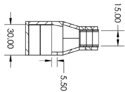
SECTION E-E
