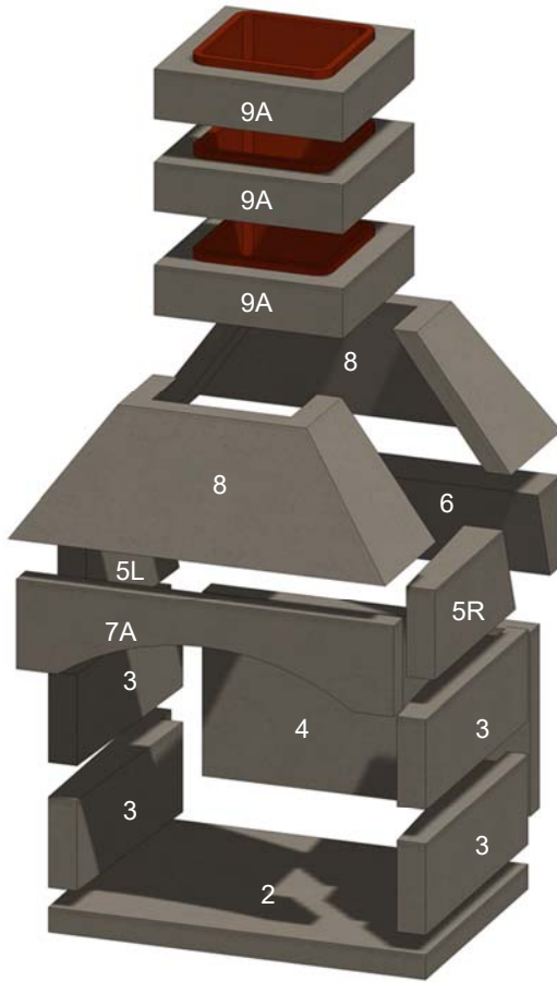
Figure 2. Fireplace Components
