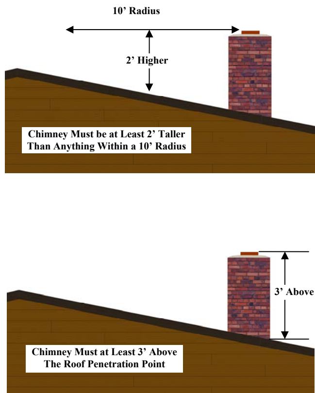
Figure 25. Chimney Height
