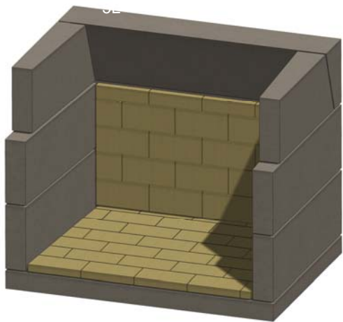
Figure 16. Back Wall Firebrick
