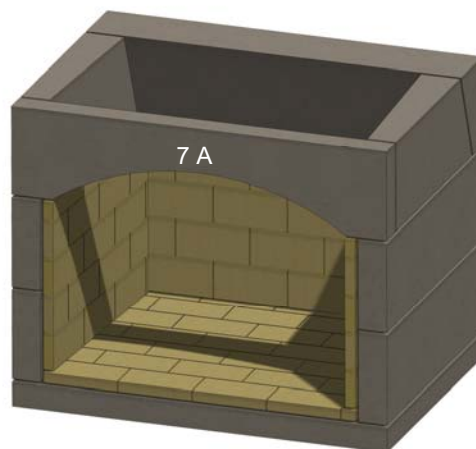
Figure 18. Front Lintel
