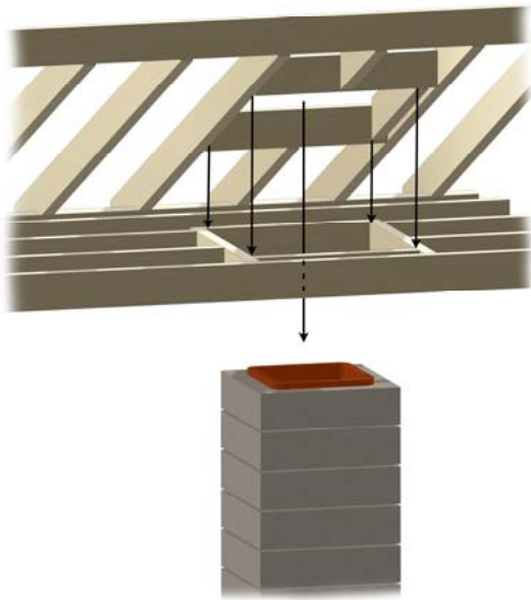
Figure 24. Roof Penetration
