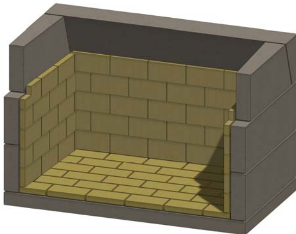
Figure 17. Sidewall Firebrick
