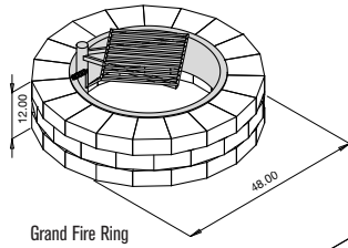
Grand Fire Ring
