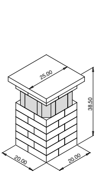
20" Pillar w/ Glass
