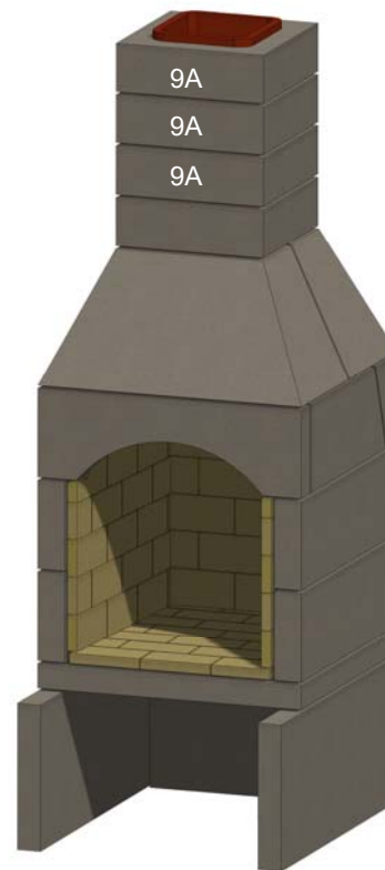
Figure 23. Chimney Complete
