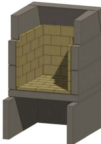
Figure 19. Sidewall Firebrick
