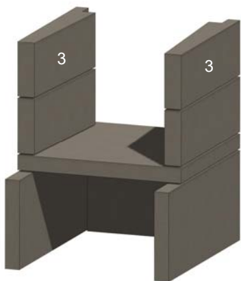
Figure 12. Middle Sidewalls
