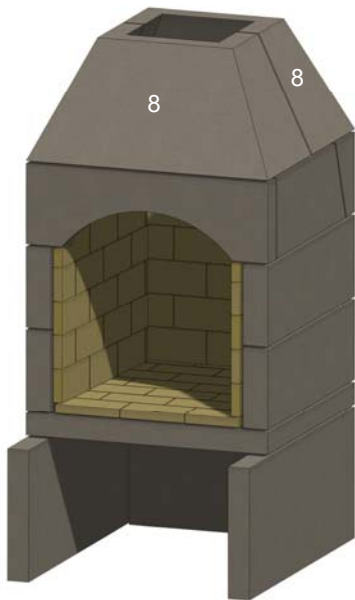
Figure 21. Throat Pieces
