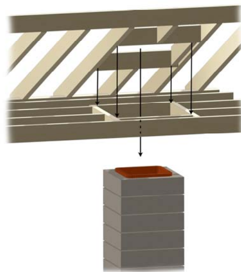
Figure 25. Roof Penetration
