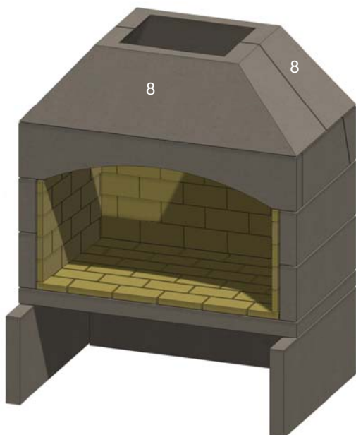
Figure 21. Throat Pieces
