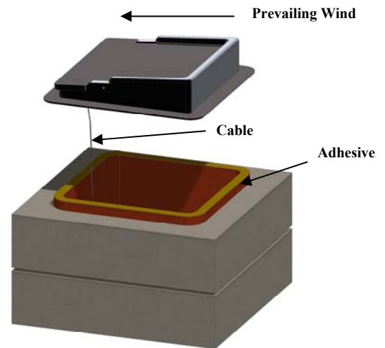
Figure 29. Install Top-Mount Damper
