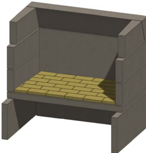
Figure 17. Floor Firebrick
