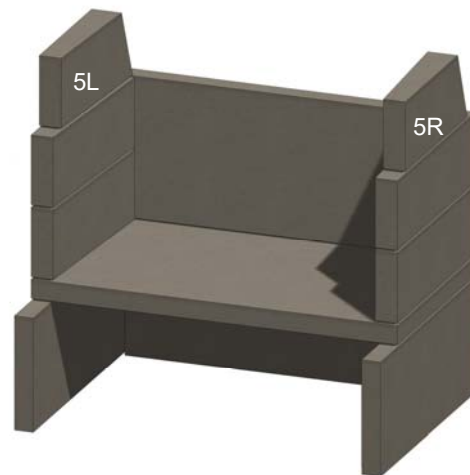
Figure 15. Upper Sidewalls
