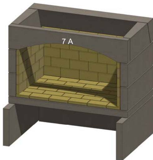
Figure 20. Front Lintel
